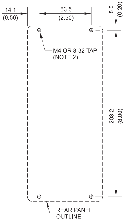
SURFACE MOUNT
