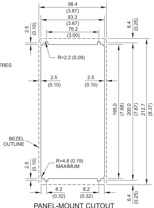
PANEL-MOUNT CUTOUT
