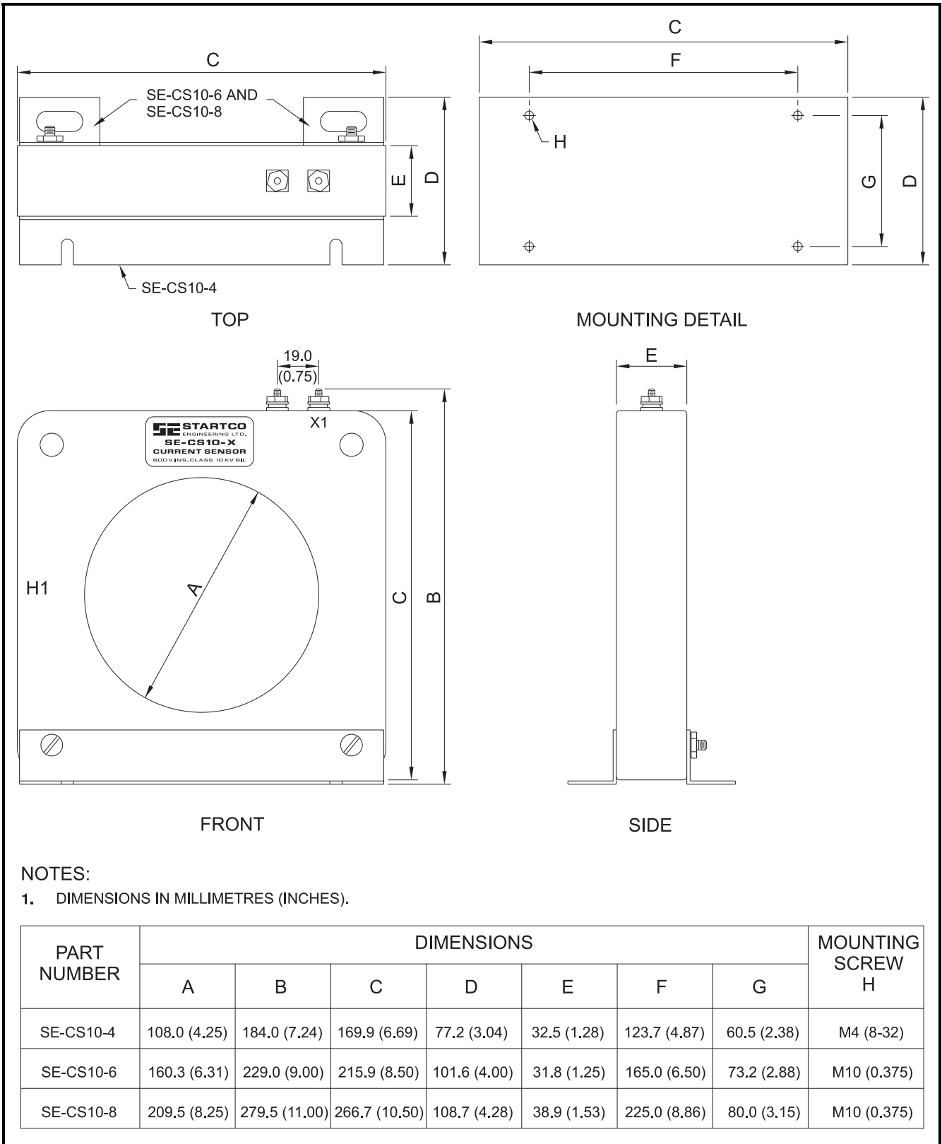
FIGURE 6. SE-CS10 Current Sensors.
