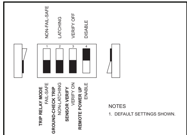
FIGURE 1. Configuration Switches.
