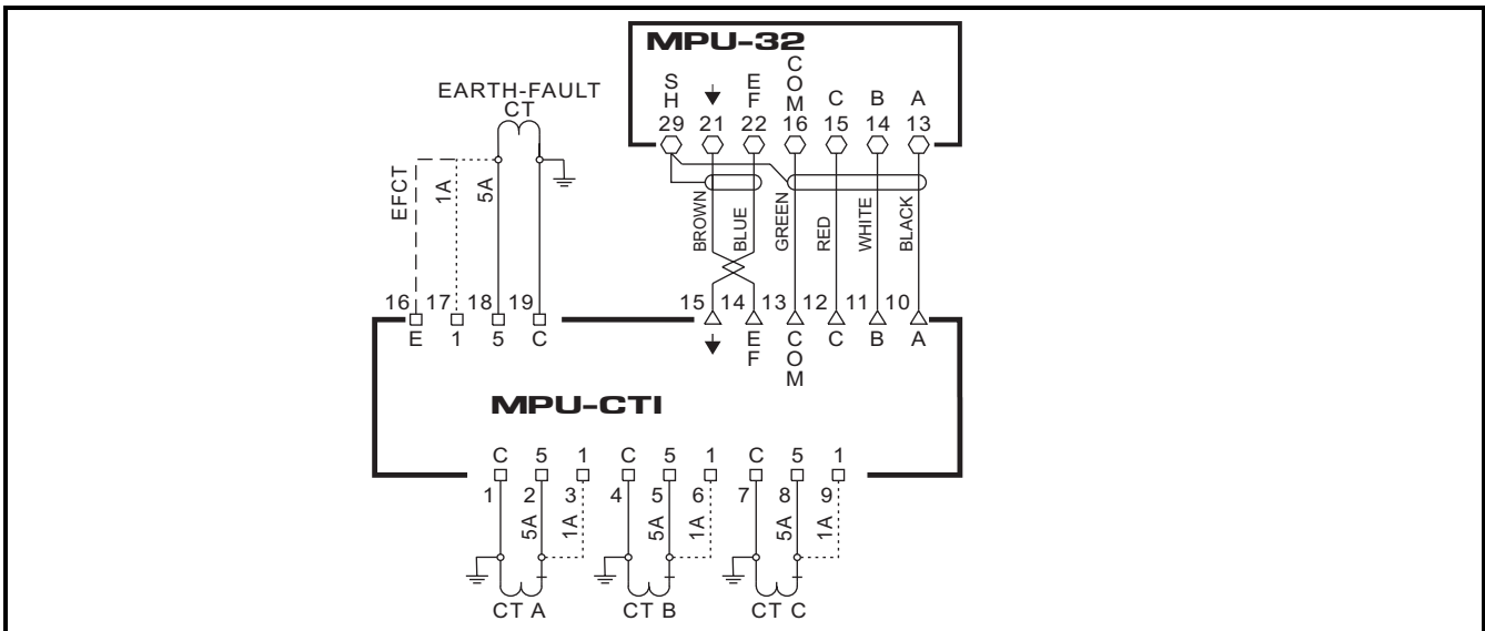
FIGURE H.4 MPU-CTI Standard Connection.
