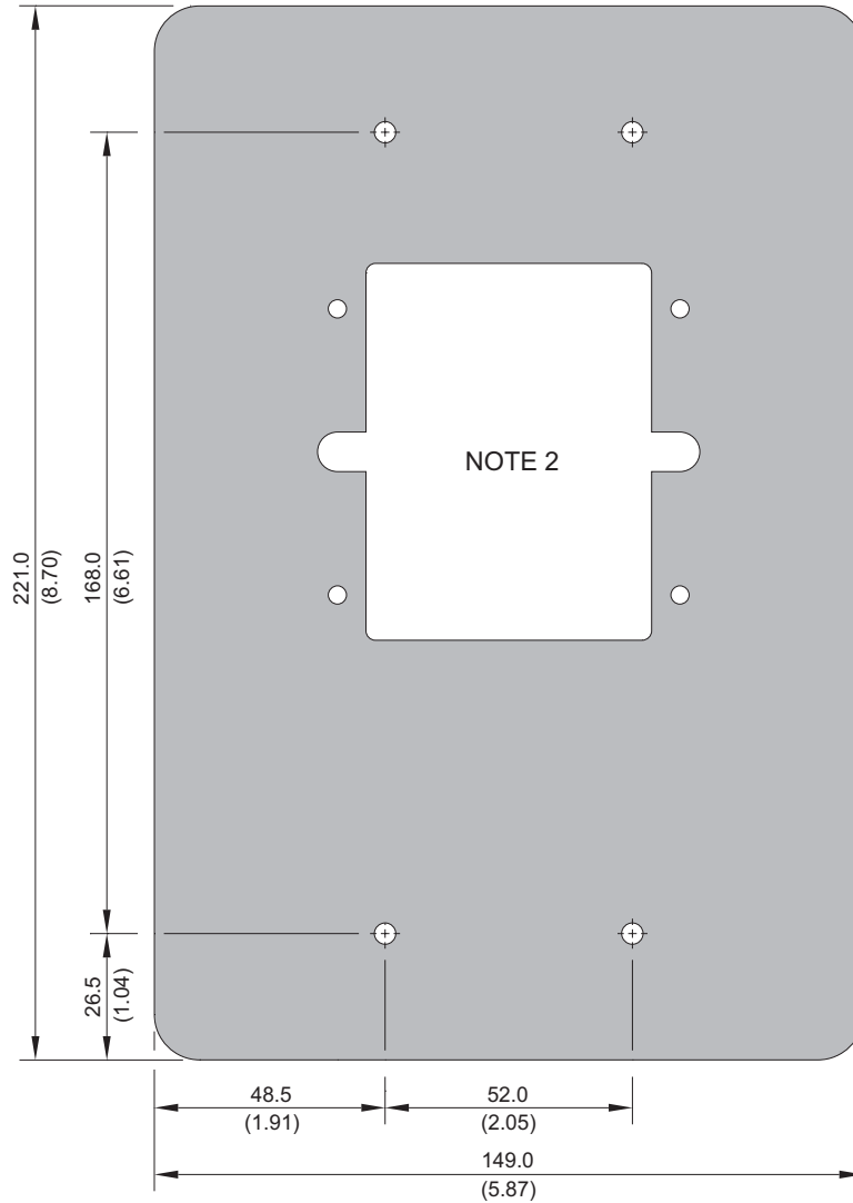
FRONT VIEW
