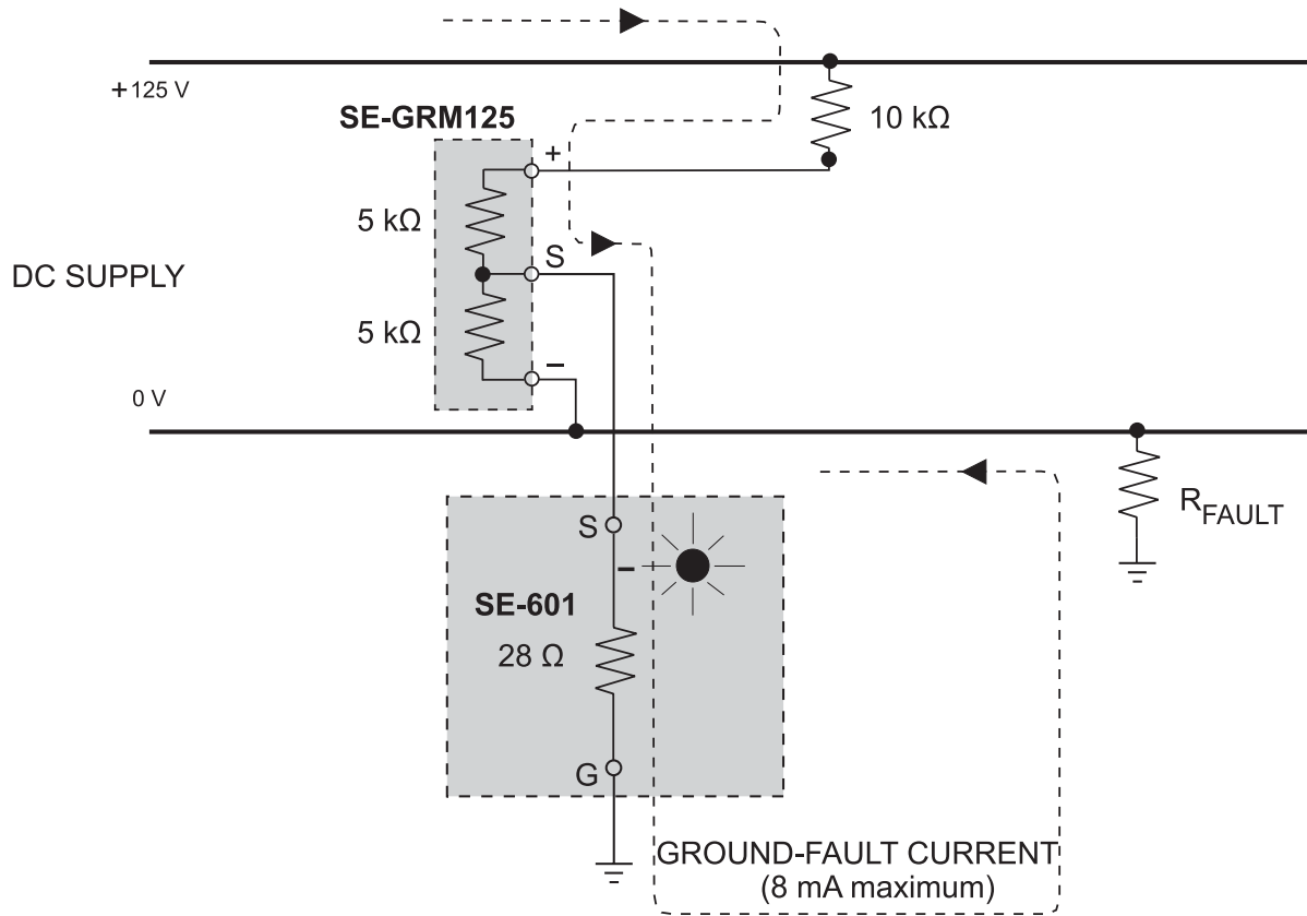
Figure 3 Fault on Negative Bus
