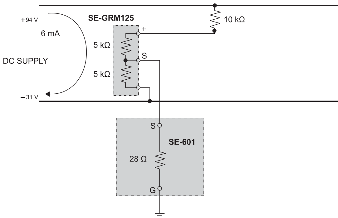
Figure 1 Unfaultered Asymmetric 125-V System
