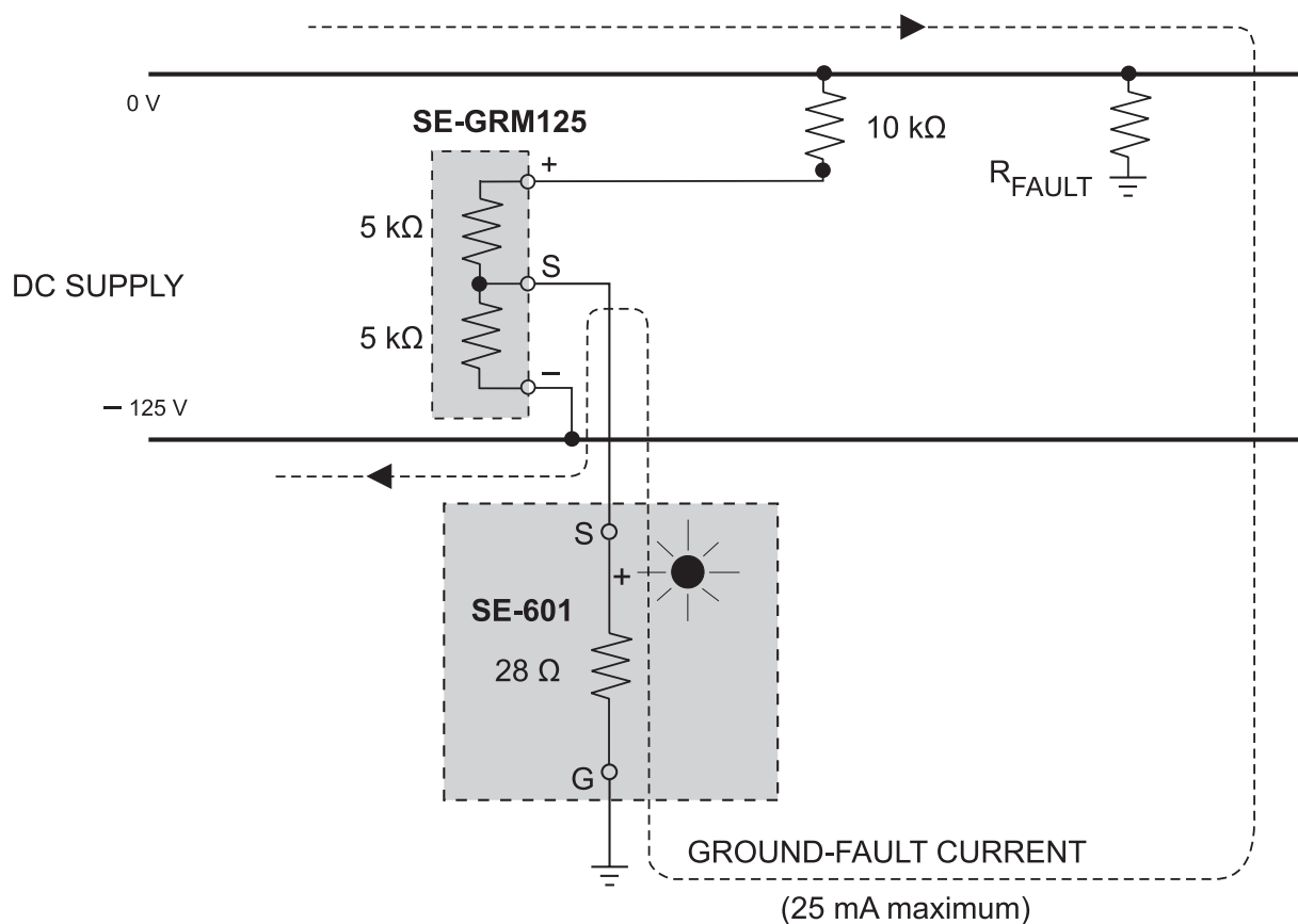
Figure 2 Fault on Positive Bus
