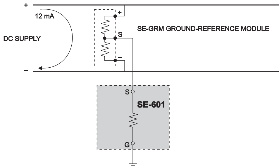
FIGURE 1. Unfaultered System
