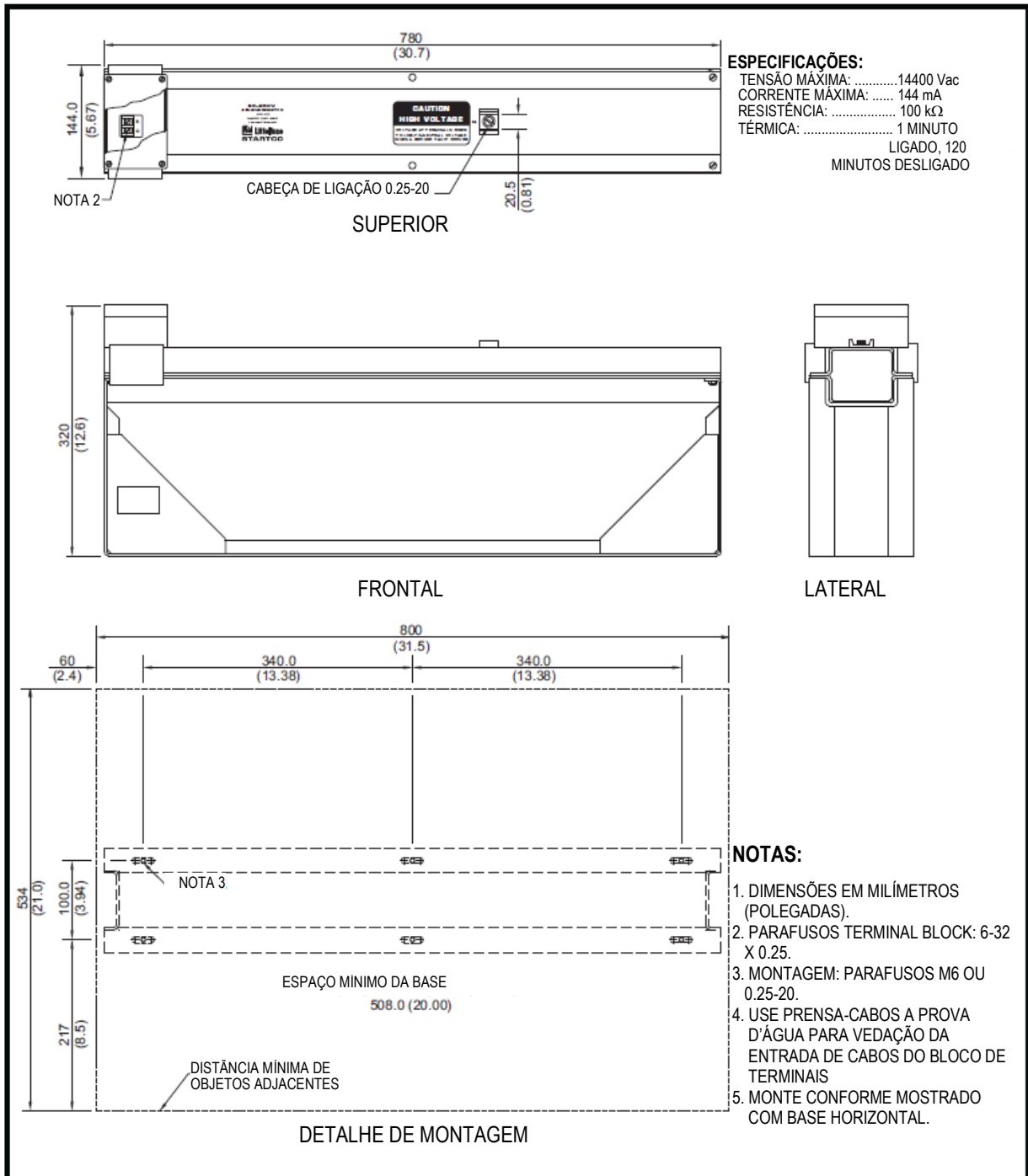
Figura 9 - ER-25KV – Resistor Sensor
