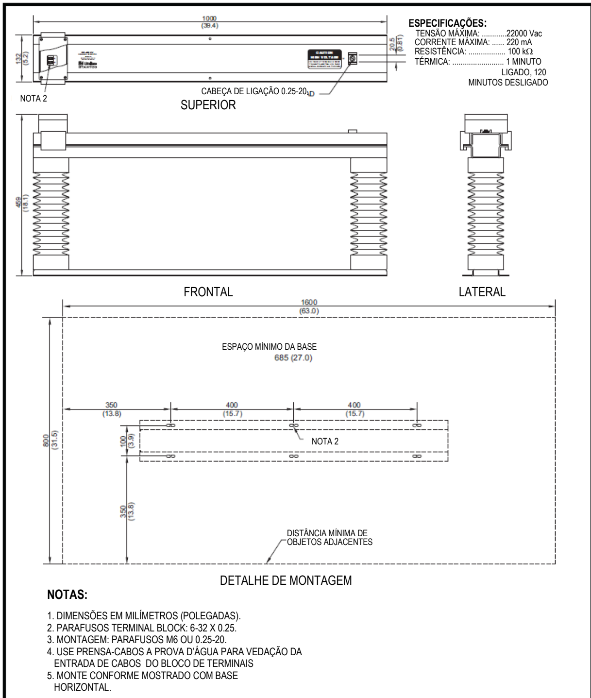
Figura 10 - ER-35KV – Resistor Sensor
