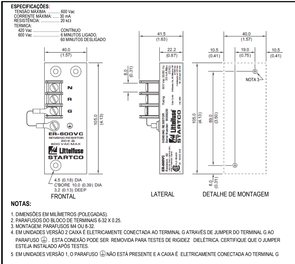
Figura 6 - ER-600VC – Resistor Sensor
