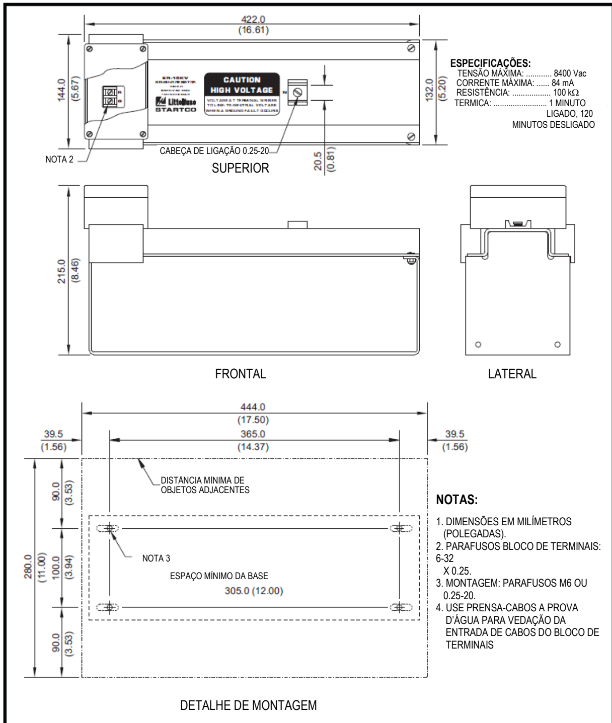
Figura 8 - ER-15KV – Resistor Sensor
