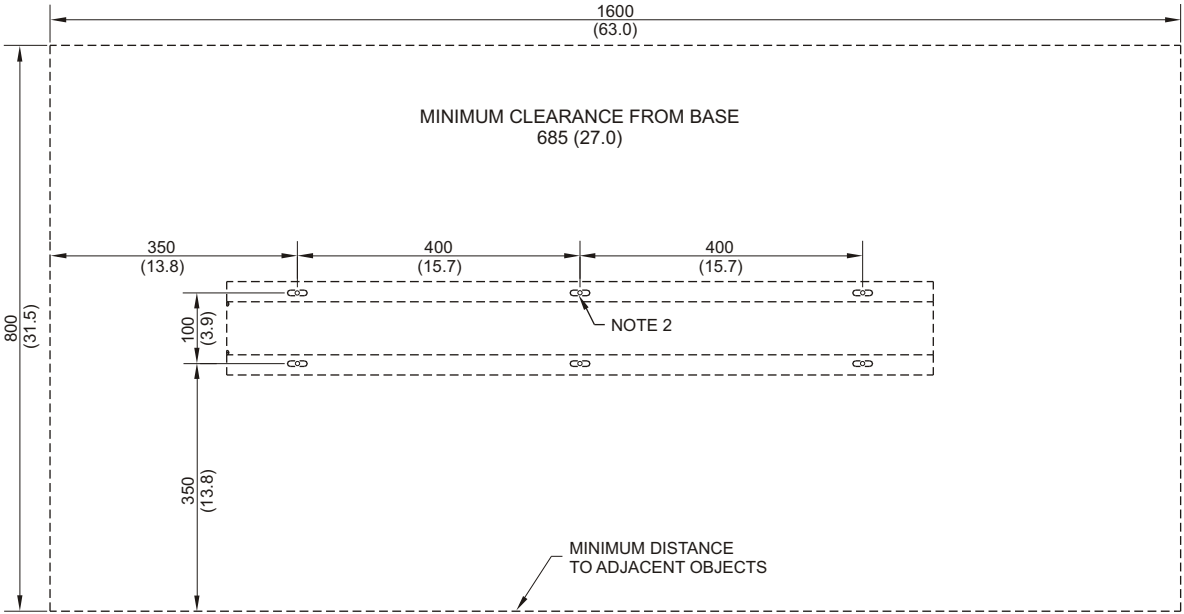
MOUNTING DETAIL
