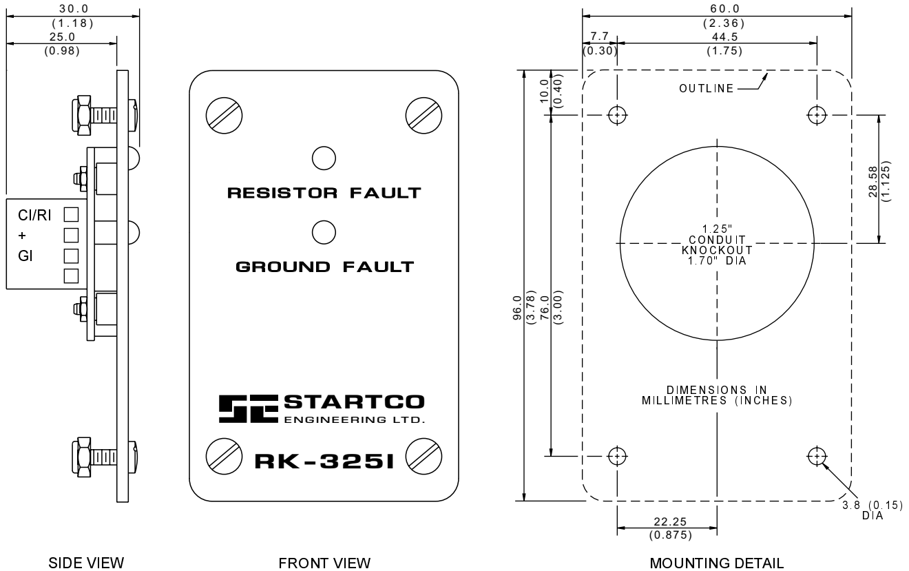
SIDE VIEW
