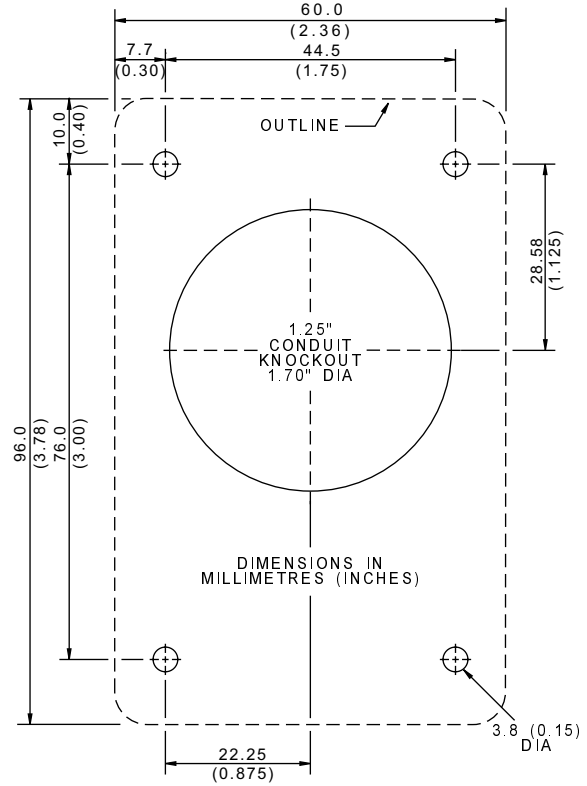
MOUNTING DETAIL
